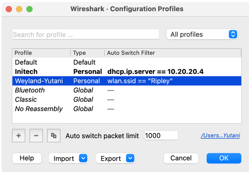
Figure 135. The configuration profiles dialog box
