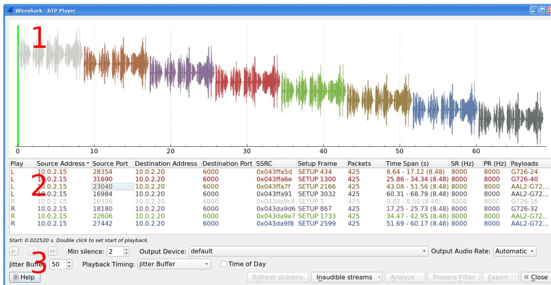
Figure 108. RTP Player window
