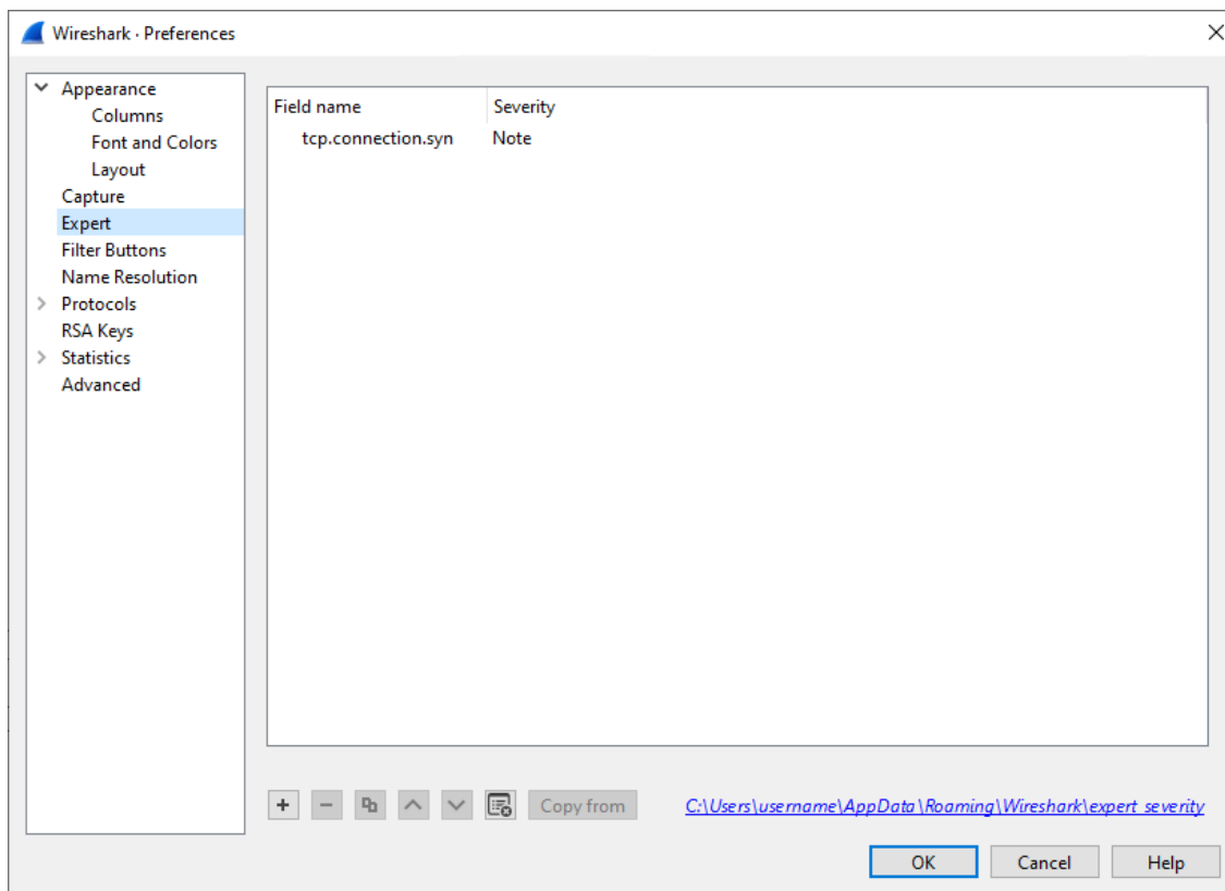
Figure 126. Expert item preferences
