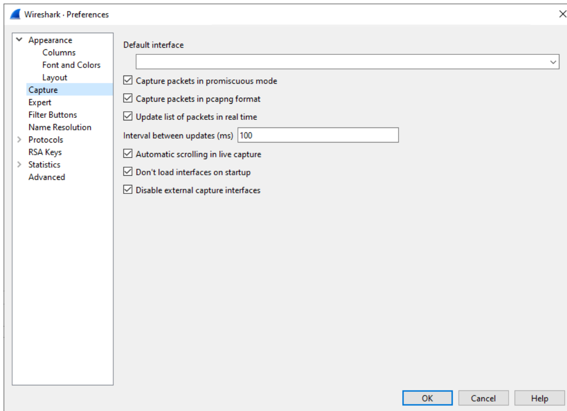
Figure 125. Capture preferences
