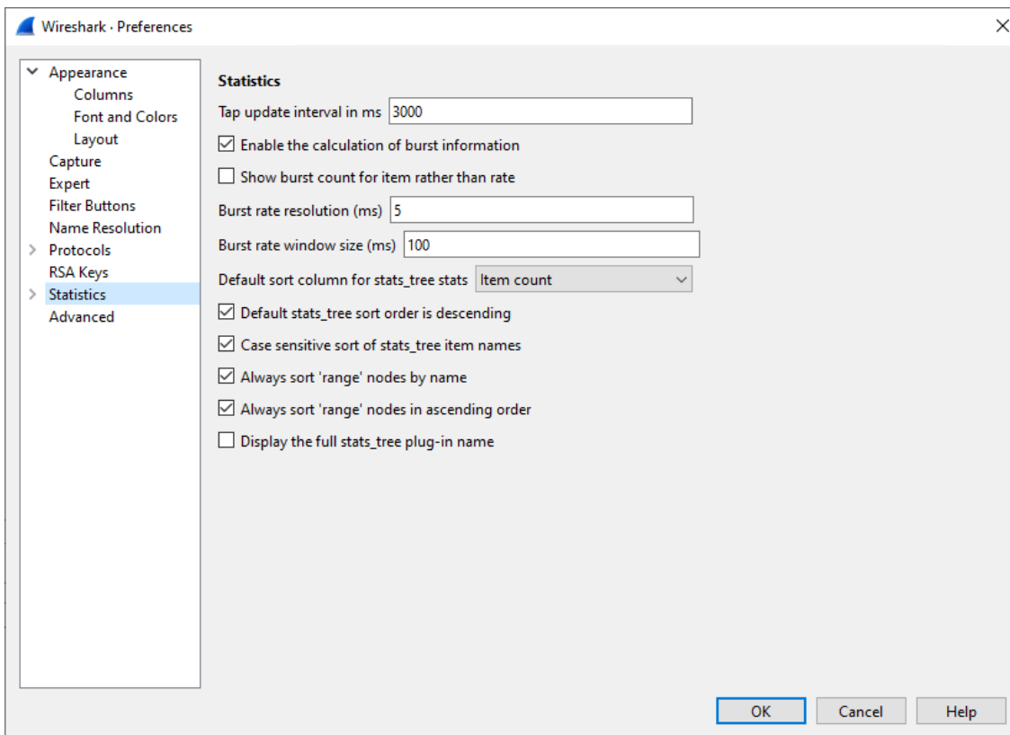
Figure 131. Statistics preferences
