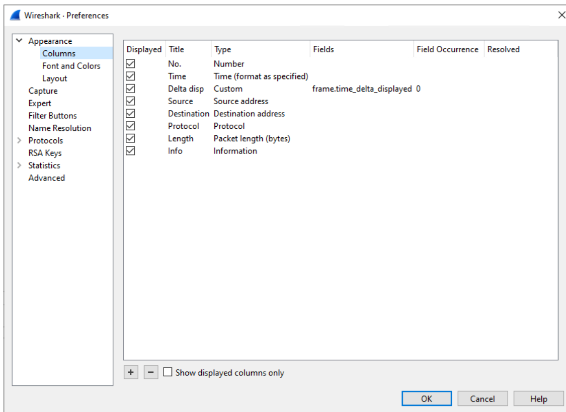
Figure 122. Column preferences
