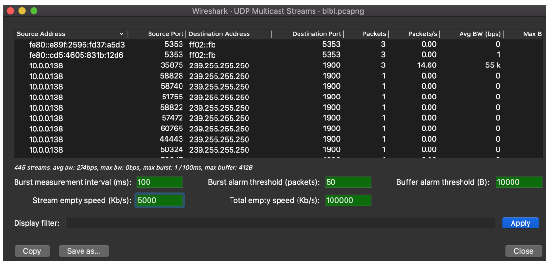
Figure 89. UDP Multicast Streams window
