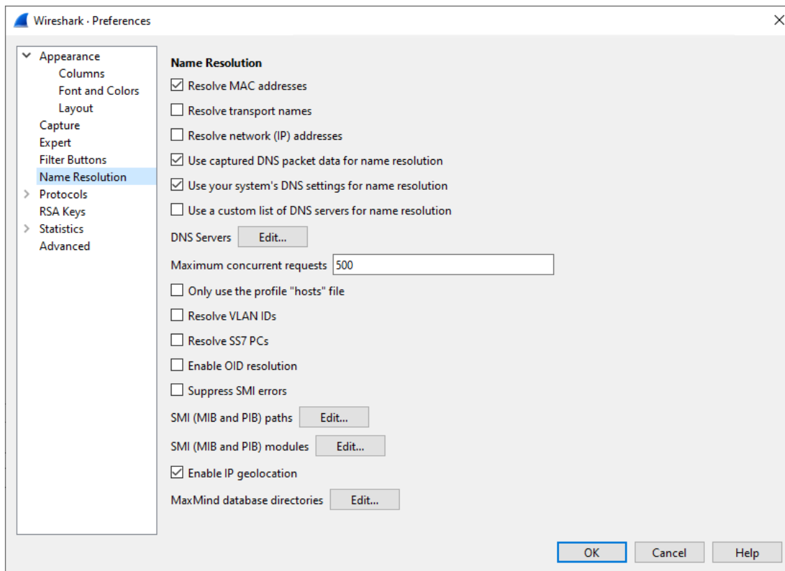
Figure 128. Name resolution preferences
