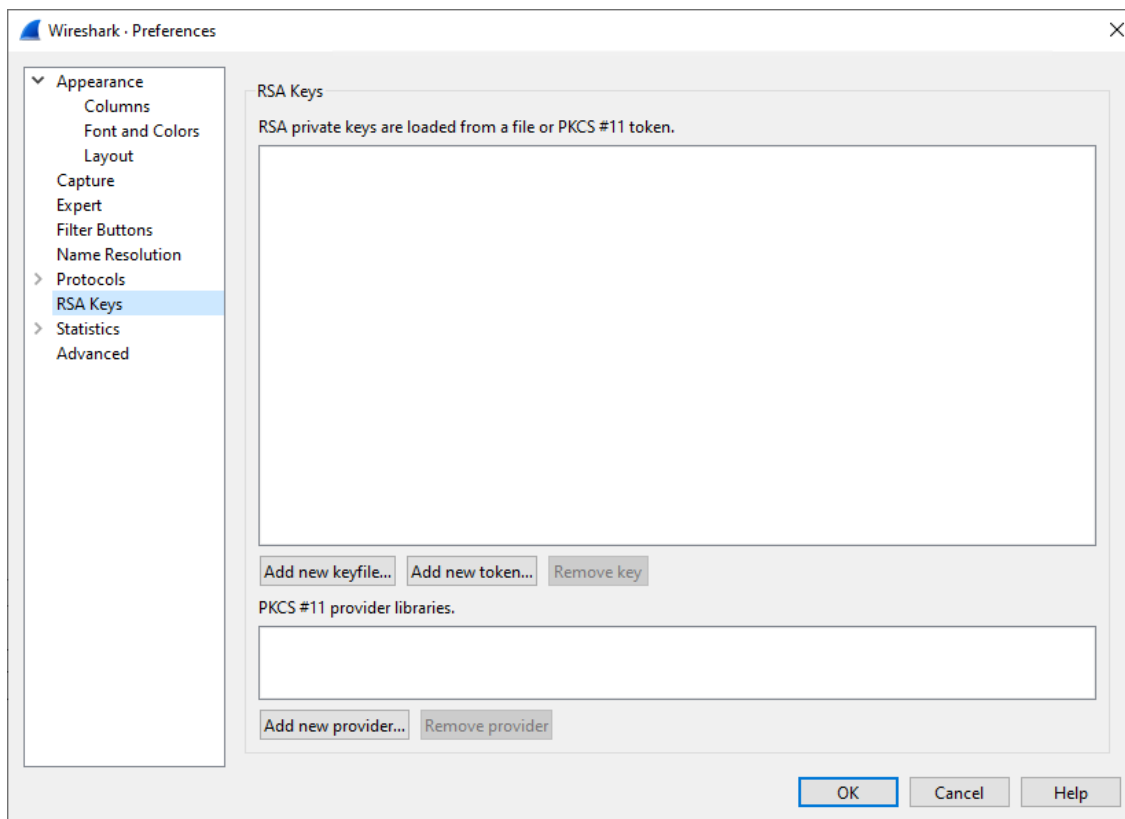
Figure 130. RSA keys
