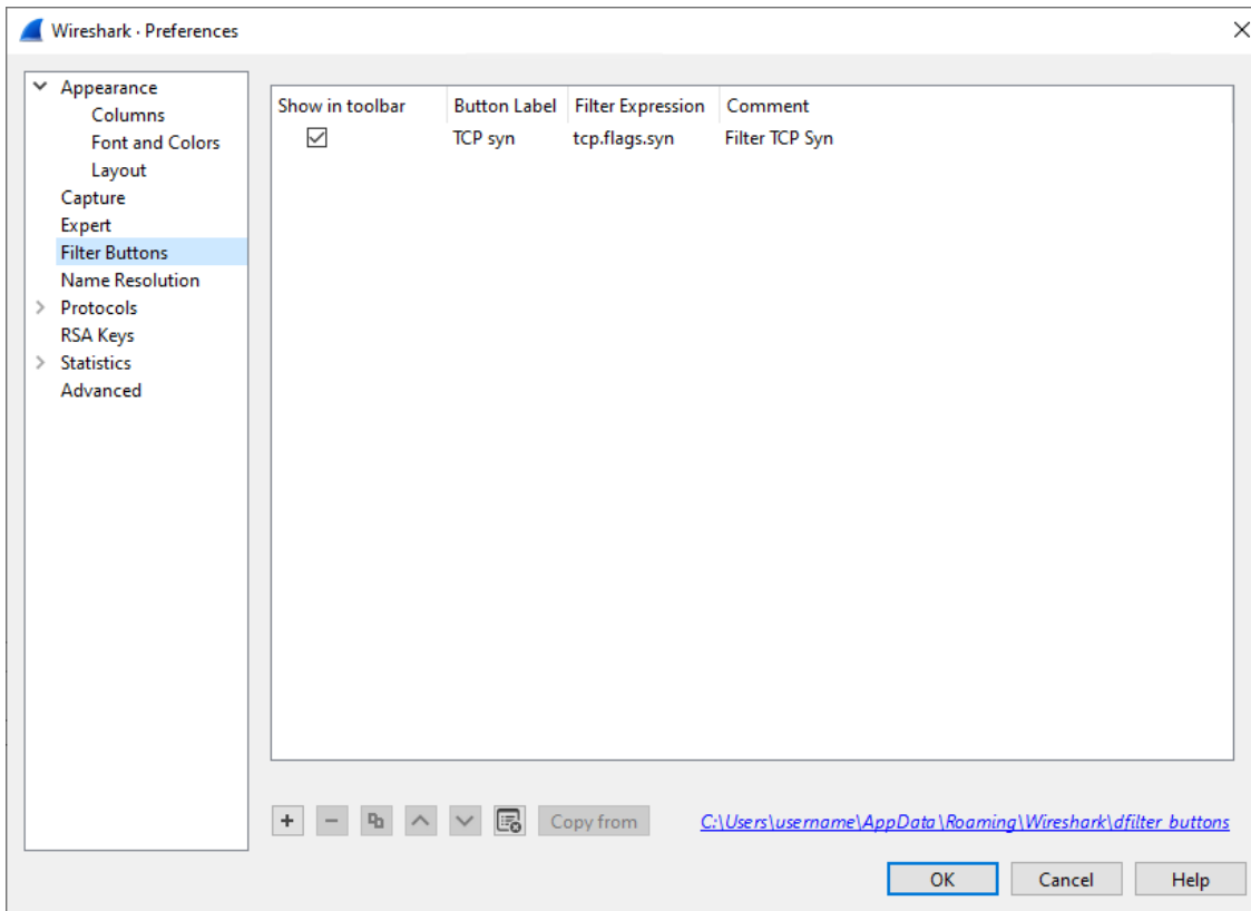
Figure 127. Filter buttons
