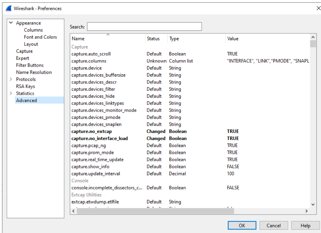
Figure 132. Advanced preferences
