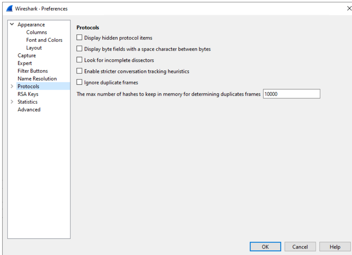
Figure 129. Protocol preferences
