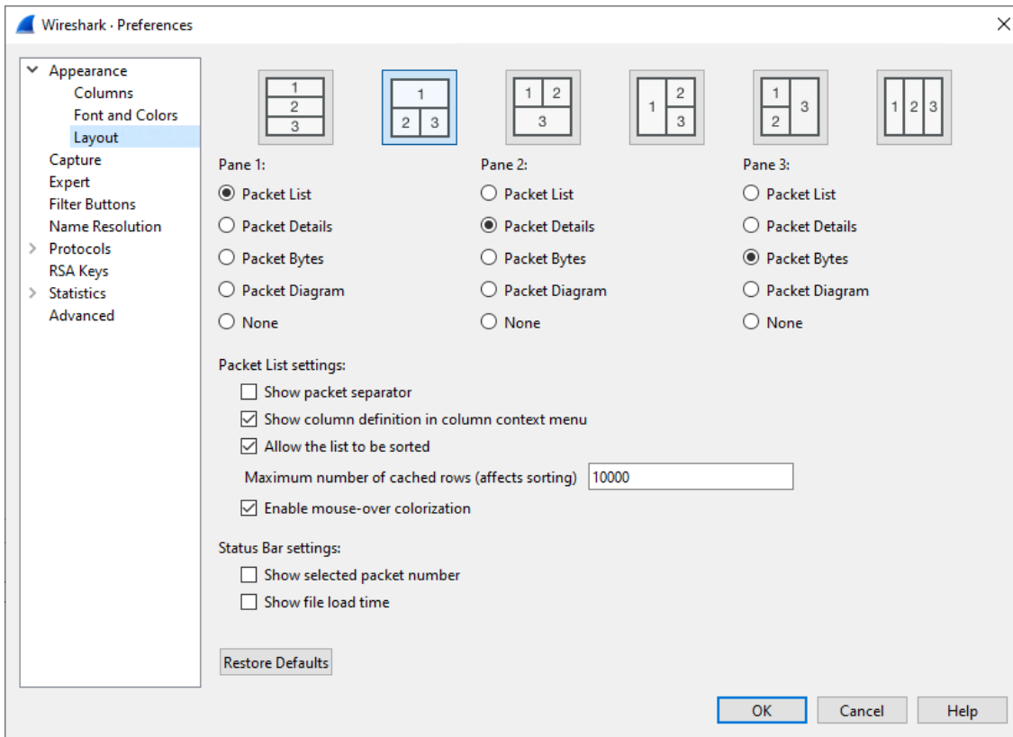
Figure 124. Layout preferences
